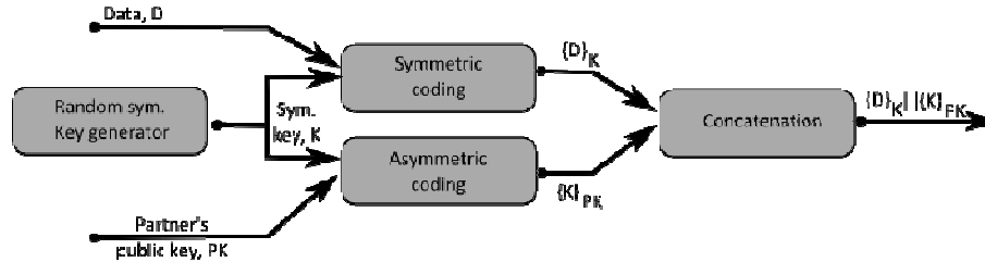
Figure 3. Encryption scheme
